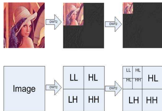
Figure 1: 2-level 2D wavelets transform
