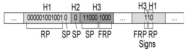
Figure 6 : Bit-stream generated from the example in the fourth bit-plane.
