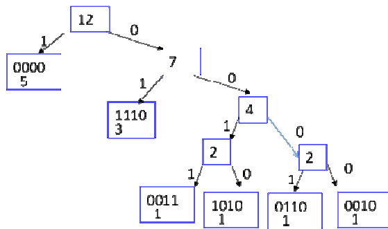
Figure 10: An example of Huffman encoding
