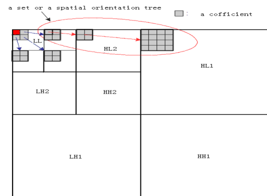
Figure2: Parent-child relationship in SPIHT
