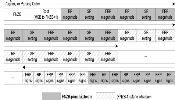
Figure 4: Bit-stream organization
